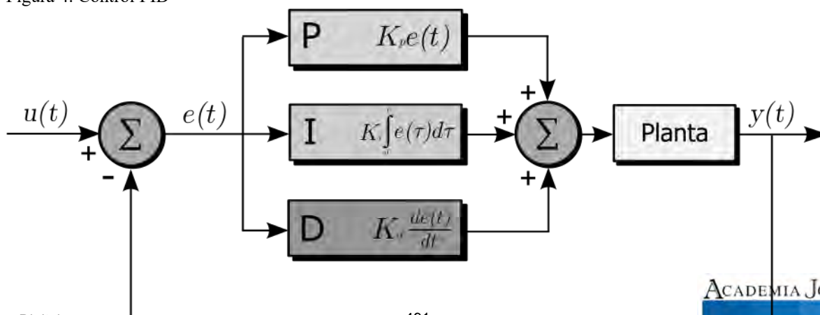
Figura 4. Control PID
