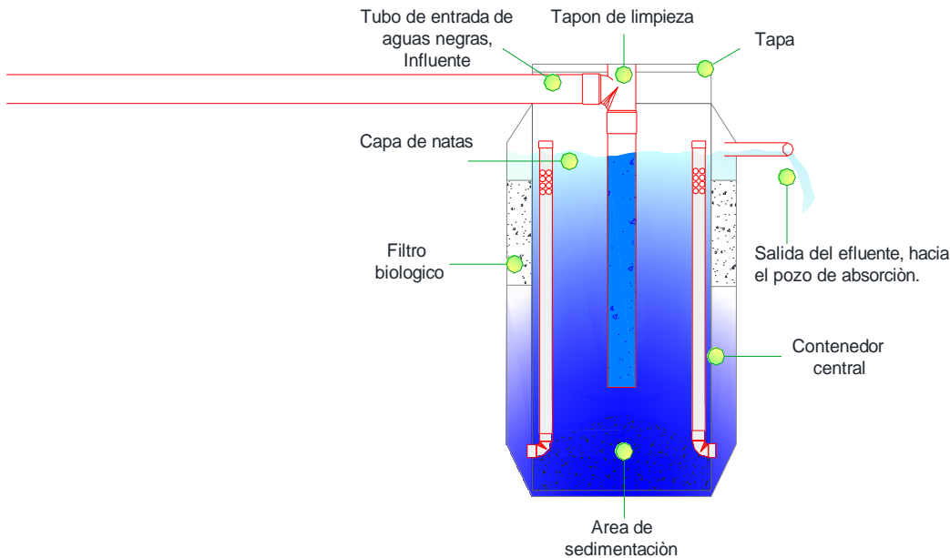
Fig 3 Biodigestor
