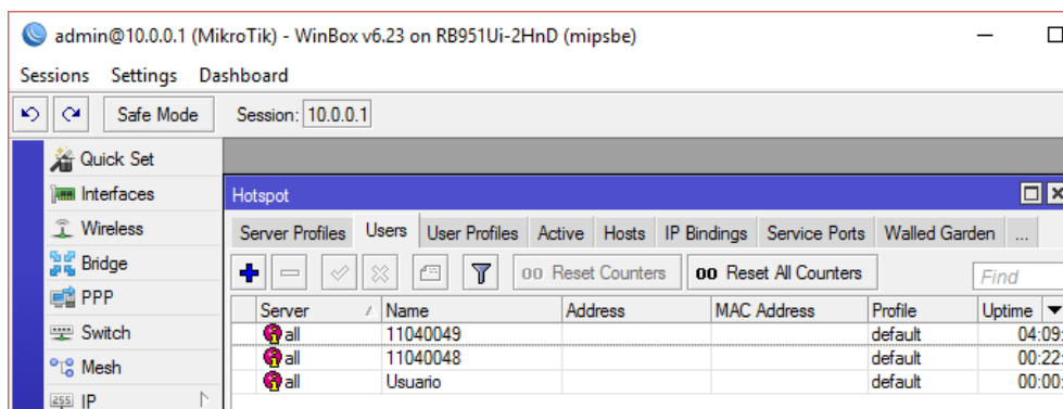
Figura 2: Interfaz Winbox
