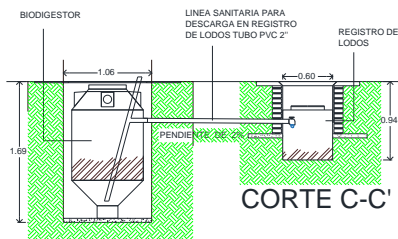
Imagen3. Planos biodigestor, 2018.
