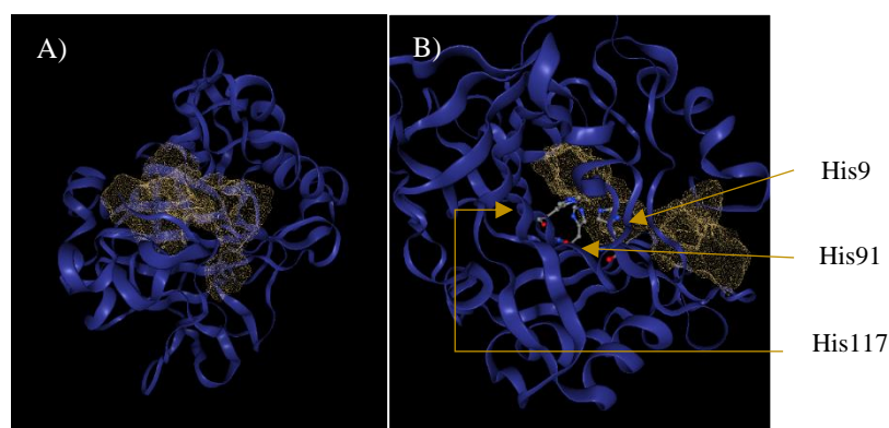
Figure 2. A) the pocket P1 yellow highlighted. B) catalytic triad of CAXII on P1.
