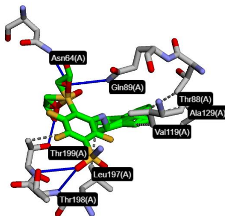
Figure 4. 6Z9 interaction fingerprint.
