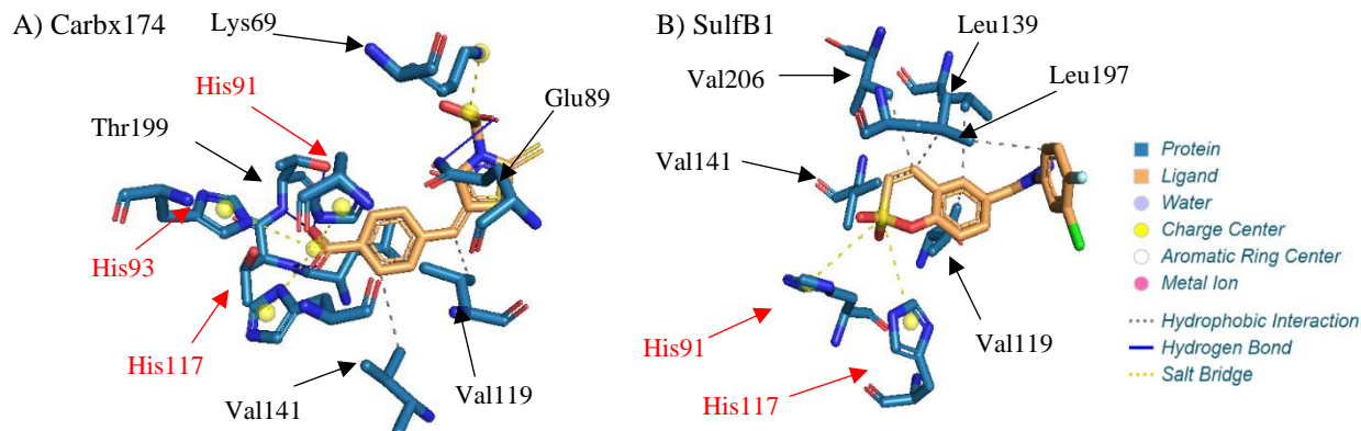
Figure 3. Compounds with the best interaction fingerprint from carboxylates and sulfocoumarins. The interesting interactions are highlighted in red. On the right is the annotation about the 3D structures.
