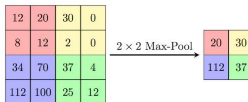
Figura 5: Max pooling
