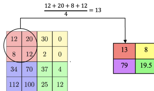
Figura 4: Average pooling
