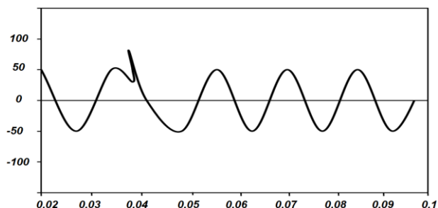
Figure 4. An impulse superposed on a voltage waveform.
